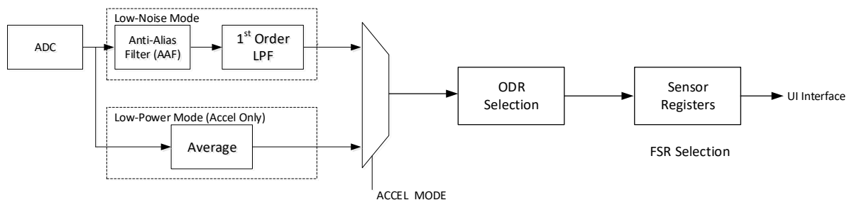
Figure 8. ICM-42670-L Signal Path
