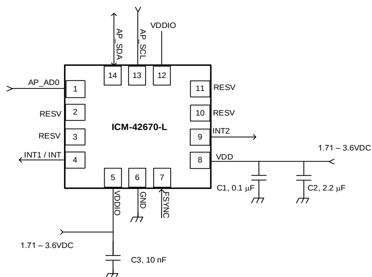
Figure 5. ICM-42670-L Application Schematic (I3C SM / I2C Interface to Host)
