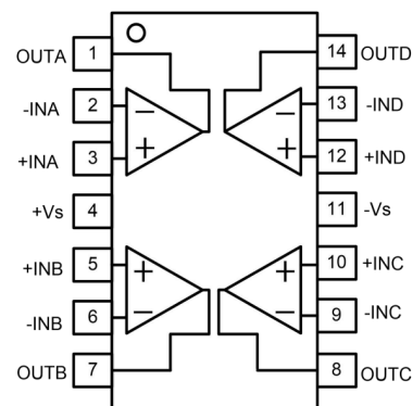
TLV9004
