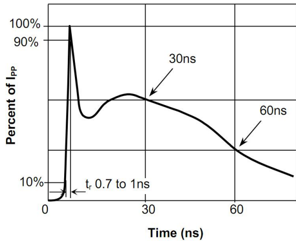
Fig.1 Pulse Waveform-ESD (IEC61000-4-2)
