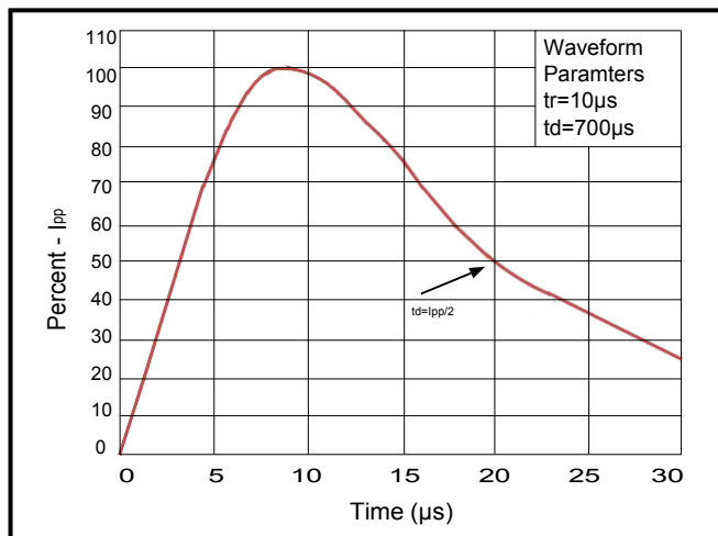
Figure 1: Pulse waveform
