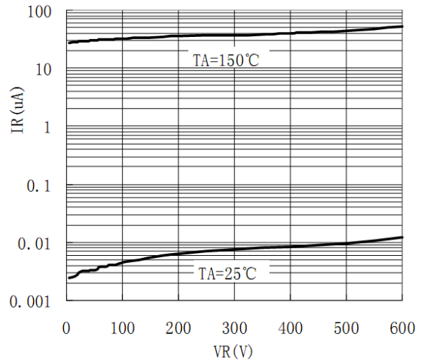
Figure 4. Reverse Characteristics
