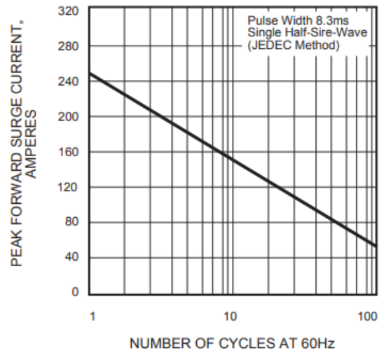
Figure 2. Peak Forward surge Current
