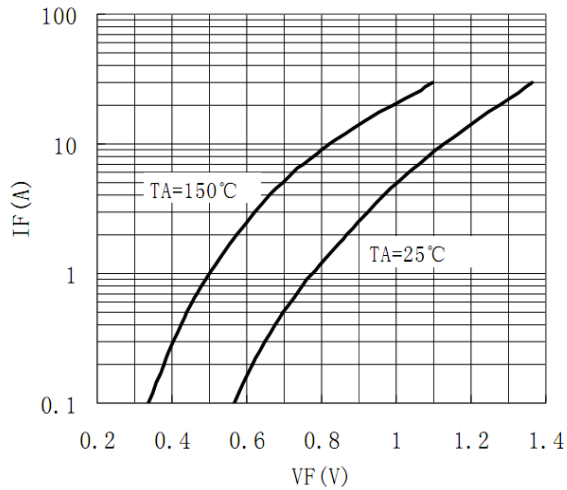
Figure 3. Forward Characteristics
