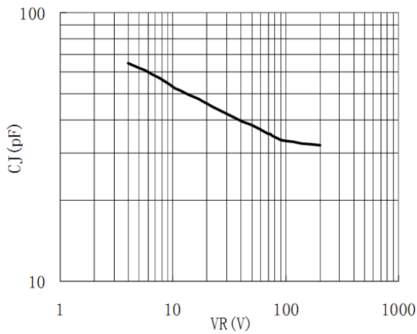
Figure 5. Junction Characteristics
