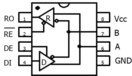
DIP-8/SOP-8
