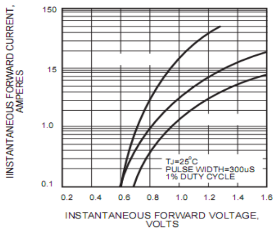
Figure 3. Forward Characteristics
