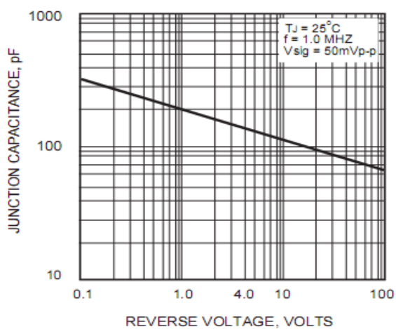
Figure 5. Junction capacitance
