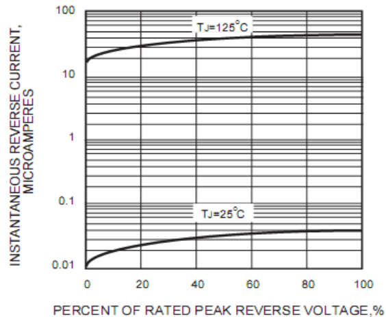
Figure 4. Reverse Characteristics
