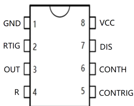
DIP-8/SOP-8
