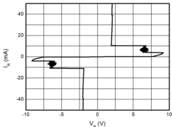
IV curve
