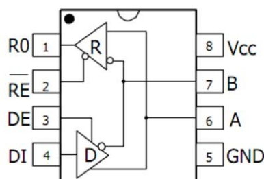
SOP-8
