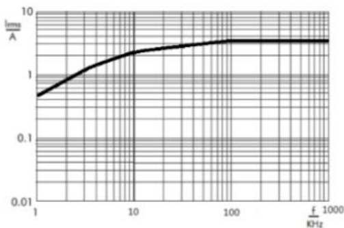
MPB-H 105J450VDC C4 Box
