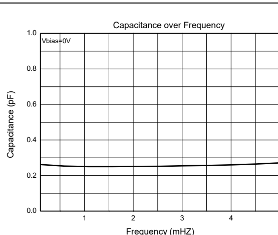
Figure6: Capacitance over Frequency
