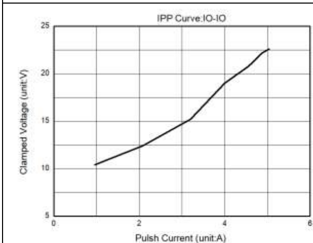
Figure3: IV Curve
