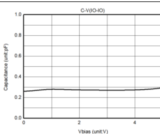
Figure2: Junction Capacitance vs. Reverse Voltage
