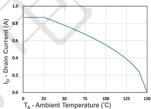
Figure 10. Drain Current
