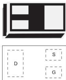
DFN1006-3L
