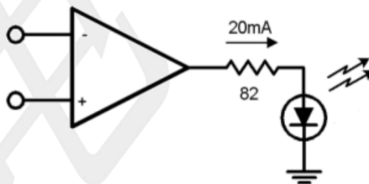
LED Driver
