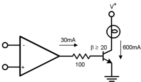
Lamp Driver
