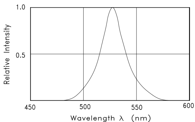
Fig.1 RELATIVE INTENSITY VS. WAVELENGTH
