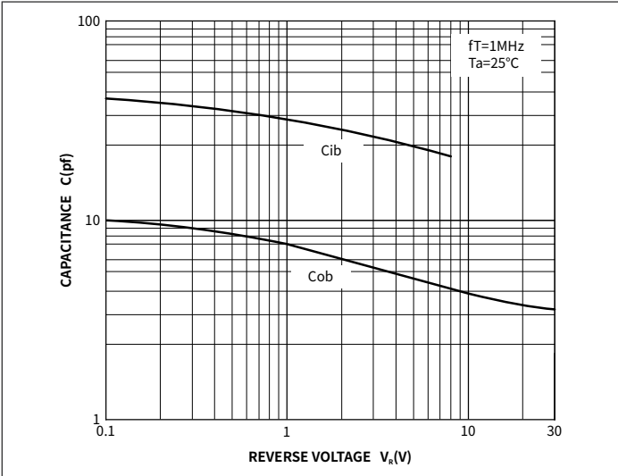
Fig.6 C_{ob}/C_{ib}-V_C V_{EB}
