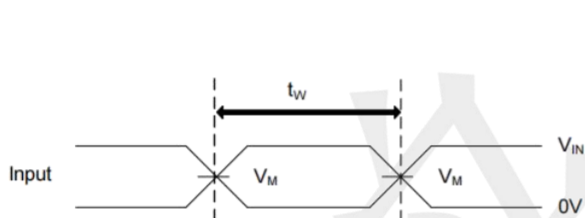
PULSE WIDTH
