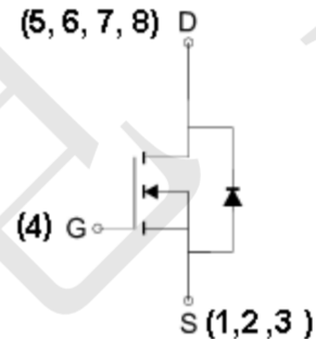
N-Channel MOSFET
