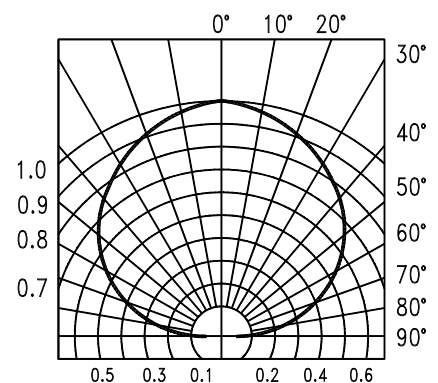
Fig.6 SPATIAL DISTRIBUTION
