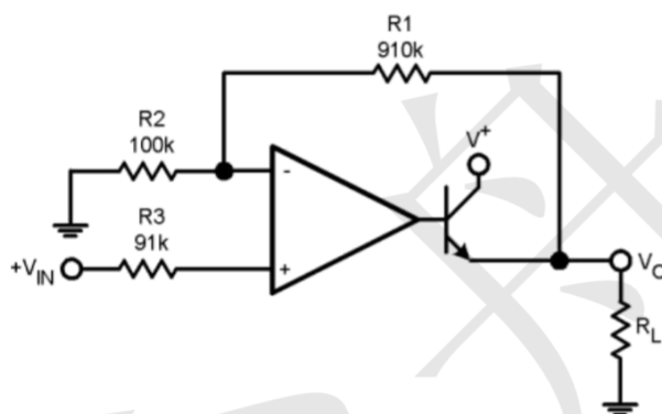
Power Amplifier
