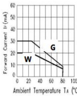
Fig.3 Forward Current Derating Curve
