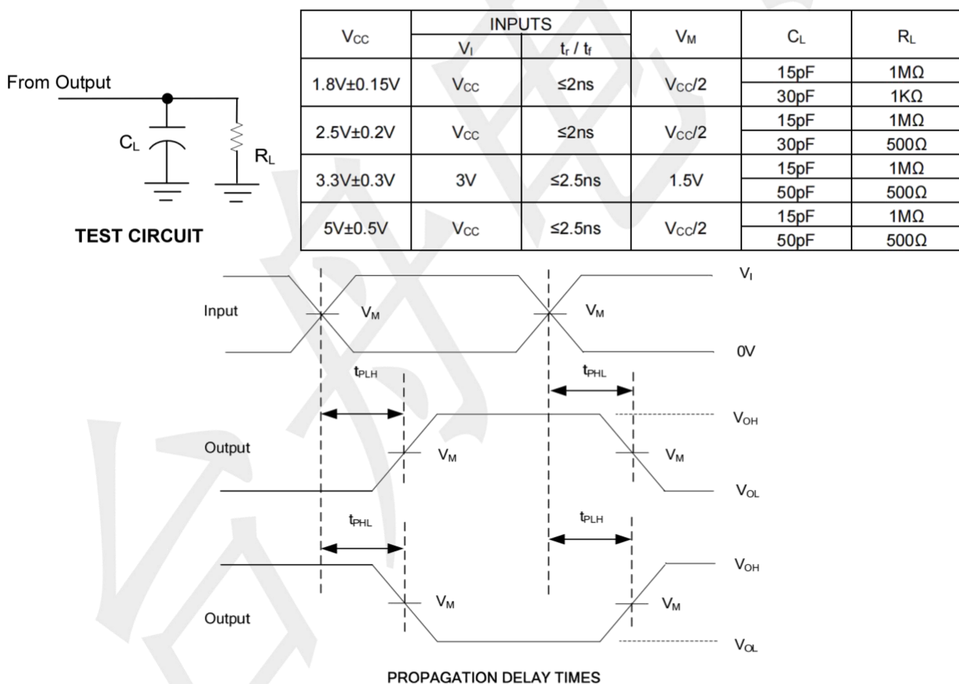
Figure 1. Test Circuit and Voltage Waveforms
