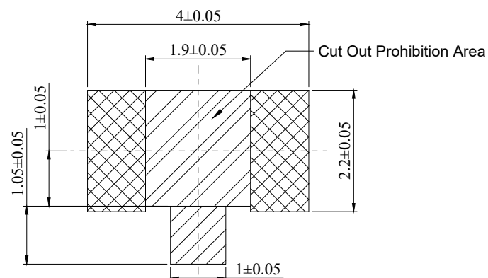
RECOMMENDED FOOTPRINT PATTERN(TOLERANCE:±0.05)
