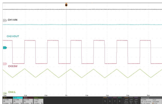
Figure 19. Switching Waveform at 0-A Load Current
