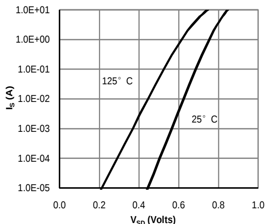
Figure 6: Body-Diode Characteristics
