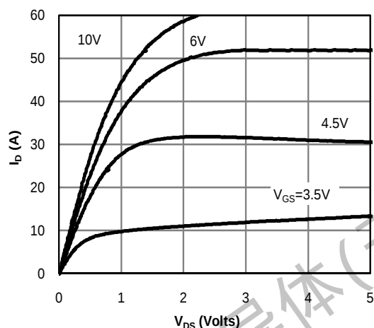
Fig 1: On-Region Characteristics
