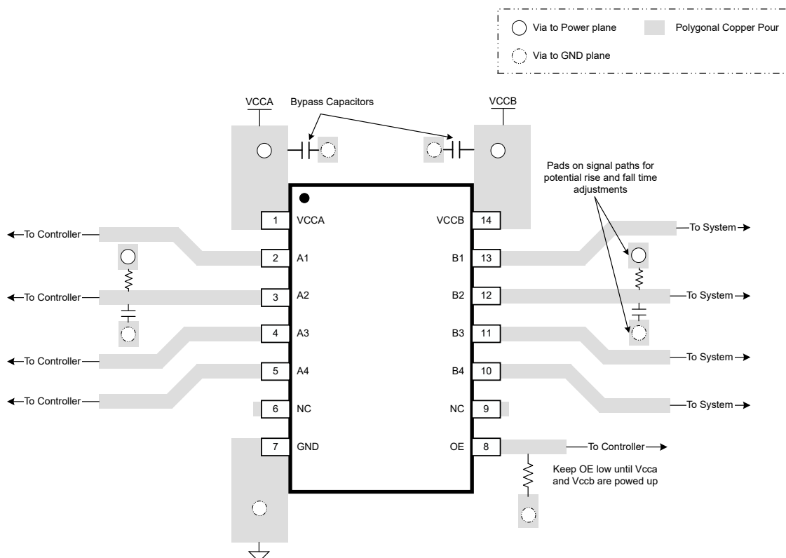
Figure 13. Layout Example
