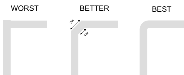
Figure 12. Trace Example
