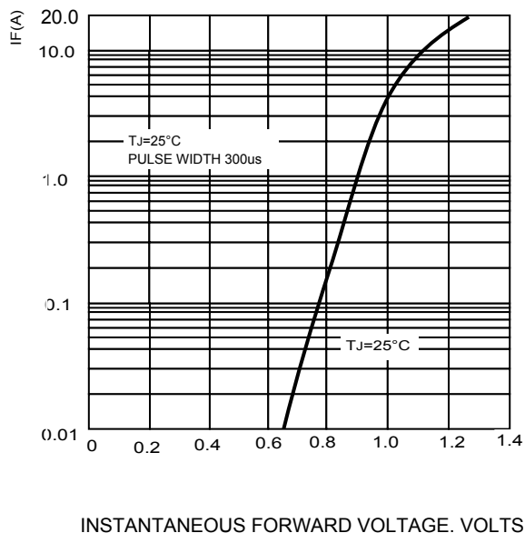
FIG.3-TYPICAL FORWARD CHARACTERISTICS
