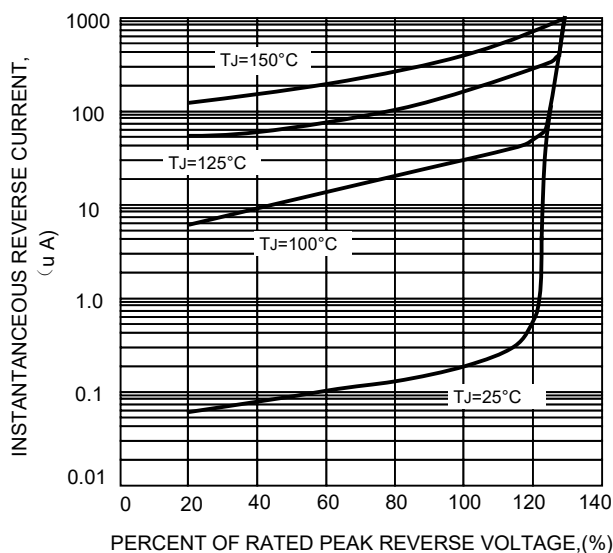
FIG.5-TYPICAL REVERSE CHARACTERISTICS
