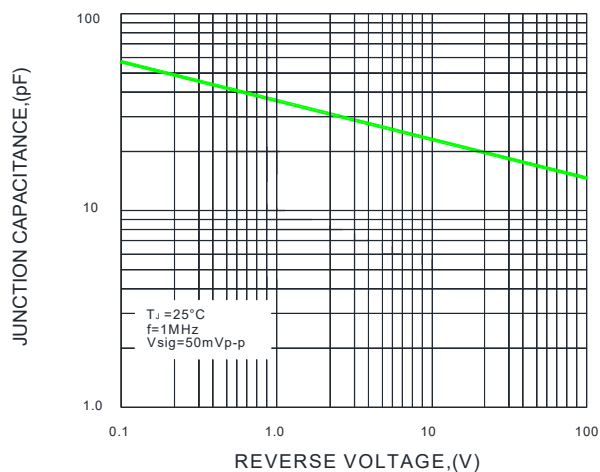
FIG.5-TYPICAL JUNCTION CAPACITANCE
