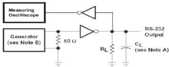
TEST CIRCUIT
