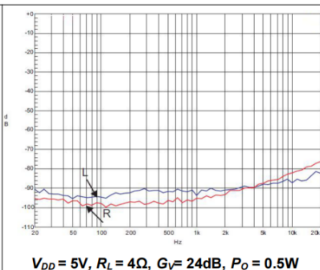
6. Crosstalk vs Frequency
