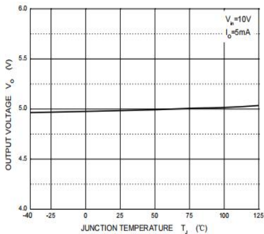
Figure 5: Temperature Characteristics
