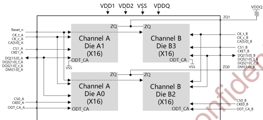
Figure 2-3 Quad-Die, Dual-Channel, Dual-Rank Package Block Diagram (8GB x32 I/O)
