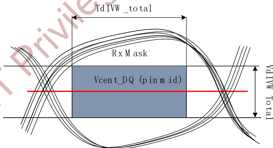
Figure 8-28 DQ Receiver(Rx) Mask
