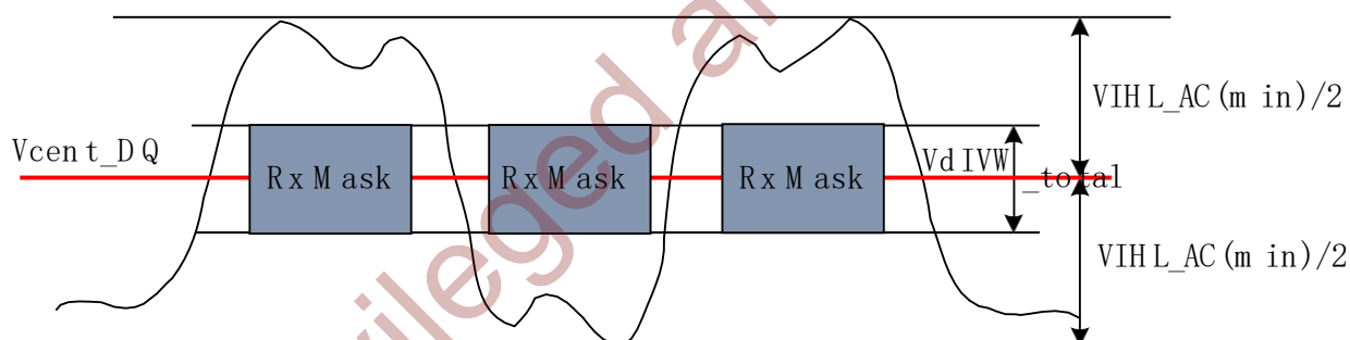
Figure 8-32 DQ VIH_L_AC definition (for Each Input Pulse)
