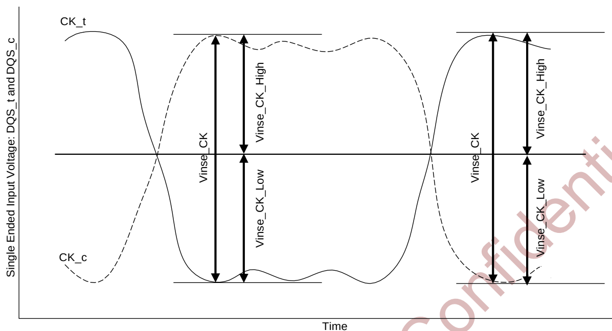
Figure 5-8 Clock Single-Ended Input Voltage
