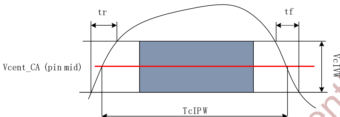
Figure 8-24 CA TcIPW and SRIN_cIVW definition (for each input pulse)
