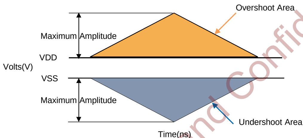
Figure 5-5 AC Overshoot and Undershoot Definition for Address and Control Pins
