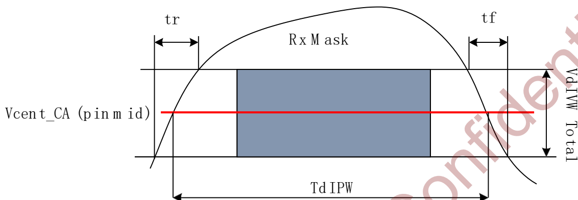
Figure 8-31 DQ TdIPW and SRIN_dIVW Definition (for Each Input Pulse)
