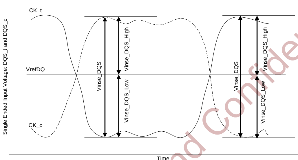
Figure 5-13 DQS Single-Ended Input Voltage
