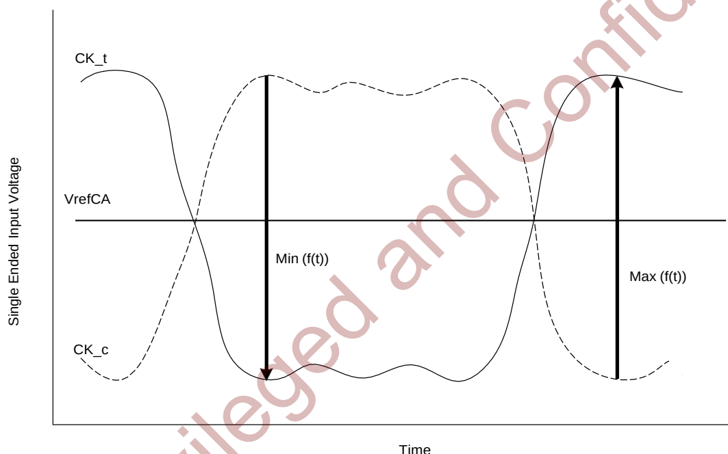
Figure 5-7 Definition of Differential Clock Peak Voltage
