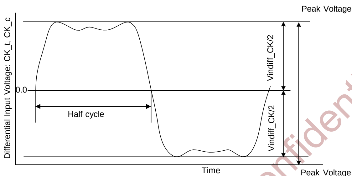
Figure 5-6 CK Differential Input Voltage
