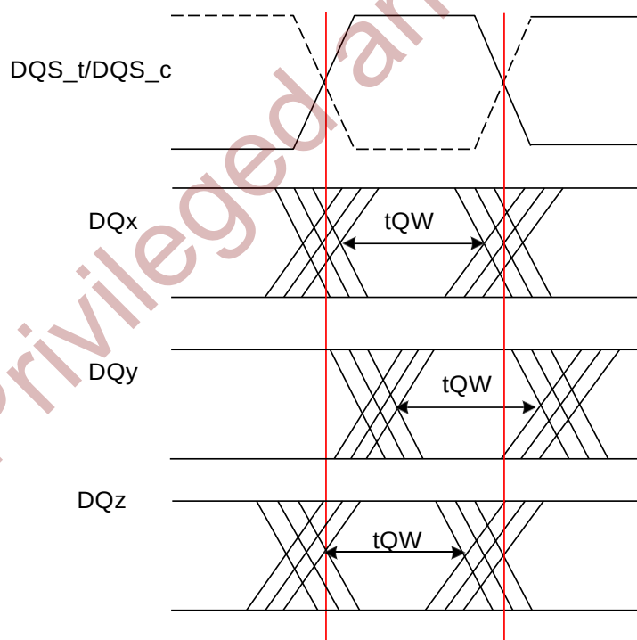
Figure 8-27 Read Data Timing t_{QW} Valid Window Defined per DQ Signal
