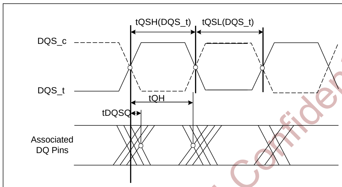
Figure 8-26 Read Data Timing Definitions t_{QH} and t_{DQSQ} across all DQ Signals per DQS Group
