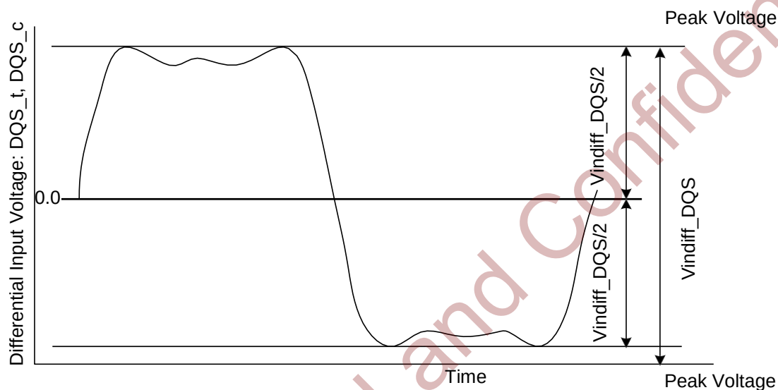
Figure 5-11 DQS Differential Input Voltage
