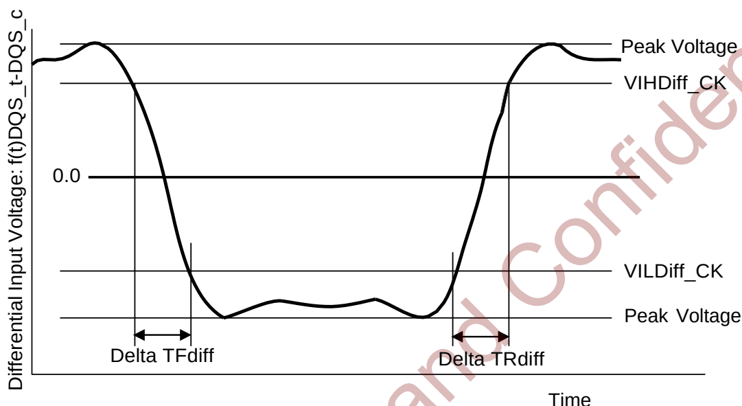
Figure 5-9 Differential Input Slew Rate Definition for CK t , CK c
