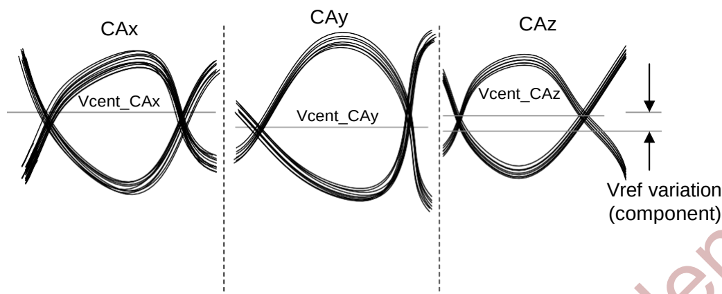
Figure 8-22 Across Pin V_{REFCA} Voltage Variation
