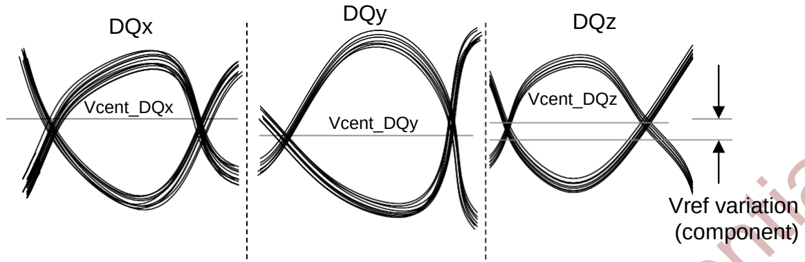
Figure 8-29 Across Pin Vref DQ Voltage Variation
