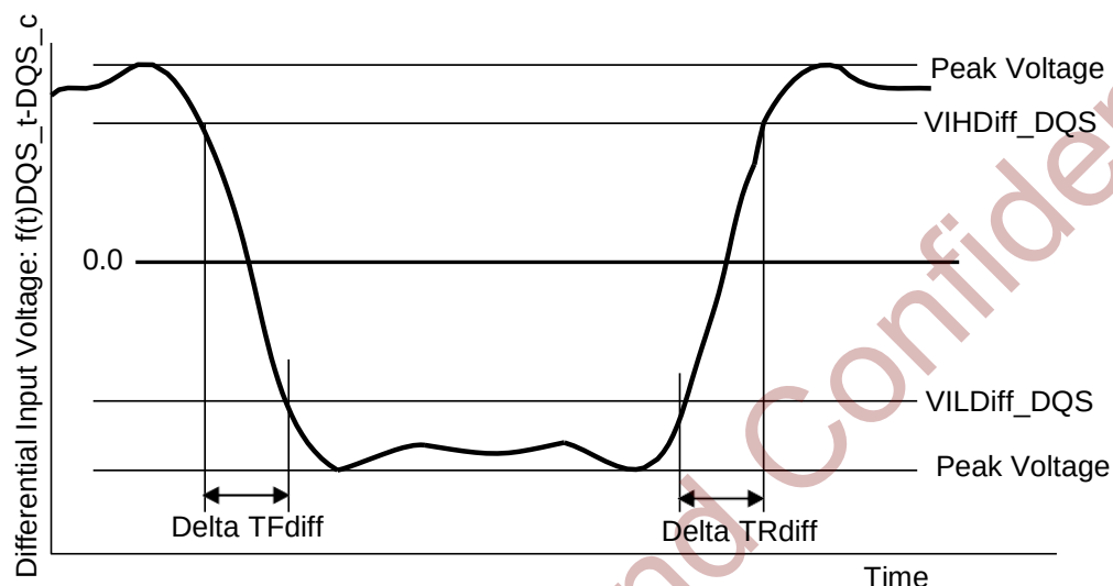
Figure 5-14 Differential Input Slew Rate Definition for DQS t , DQS c
