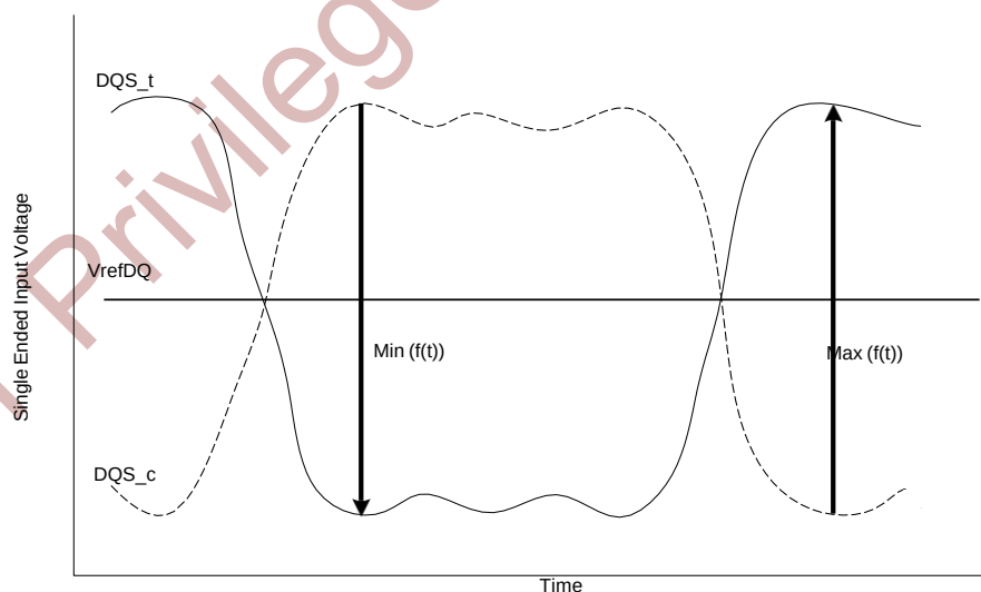
Figure 5-12 Definition of Differential DQS Peak Voltage
