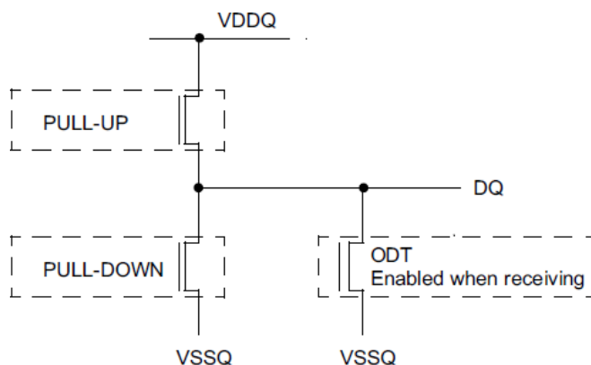
Figure 5-18 LVSTL I/O Cell
