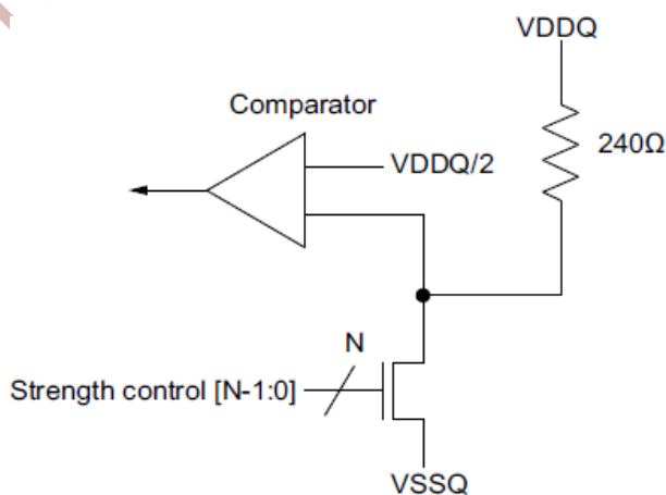
Figure 5-19 Pull-down Calibration
