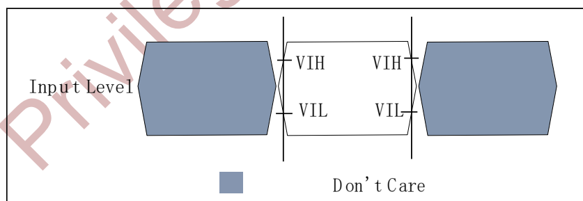
Figure 5-4 Input AC Timing Definition for Reset_n and ODT_CA
