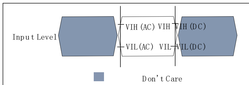
Figure 5-3 Input AC Timing Definition for CKE
