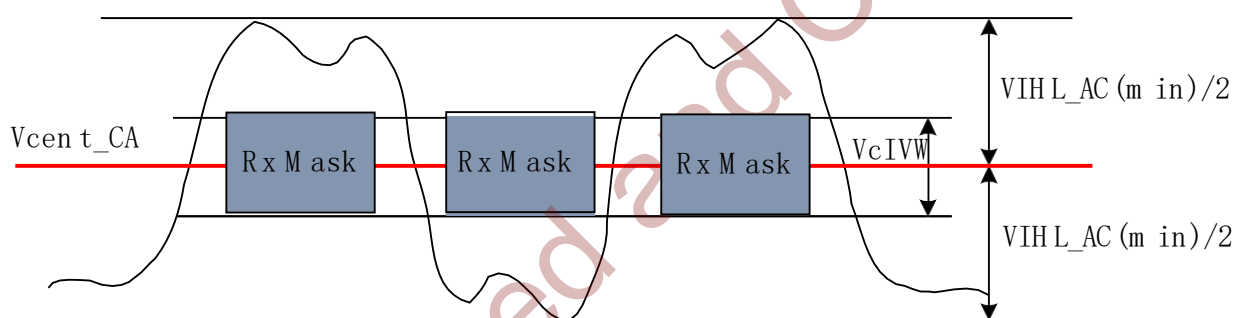
Figure 8-25 CA VIH_L_AC Definition (for Each Input Pulse)
