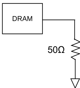
Figure 5-17 Driver Output Reference Load for Timing and Slew Rate
