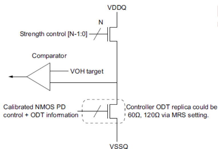
Figure 5-20 Pull-up Calibration
