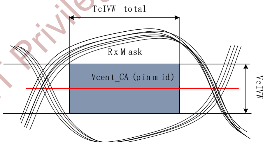
Figure 8-21 CA Receiver(Rx) Mask
