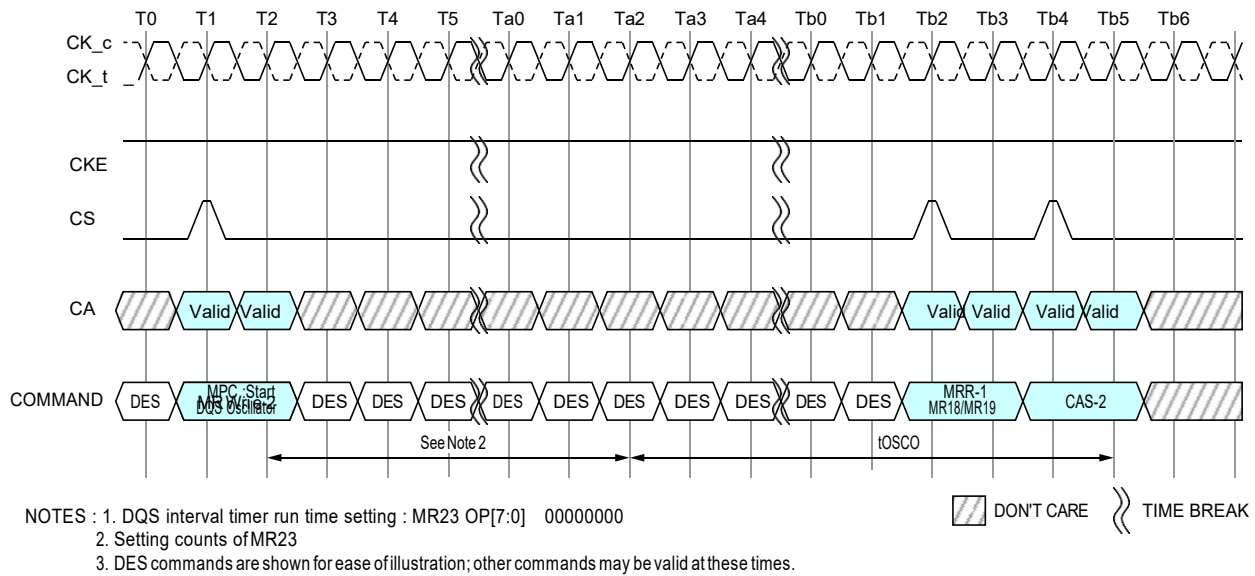
Figure - In case of DQS Interval Oscillator is stopped by DQS interval timer
