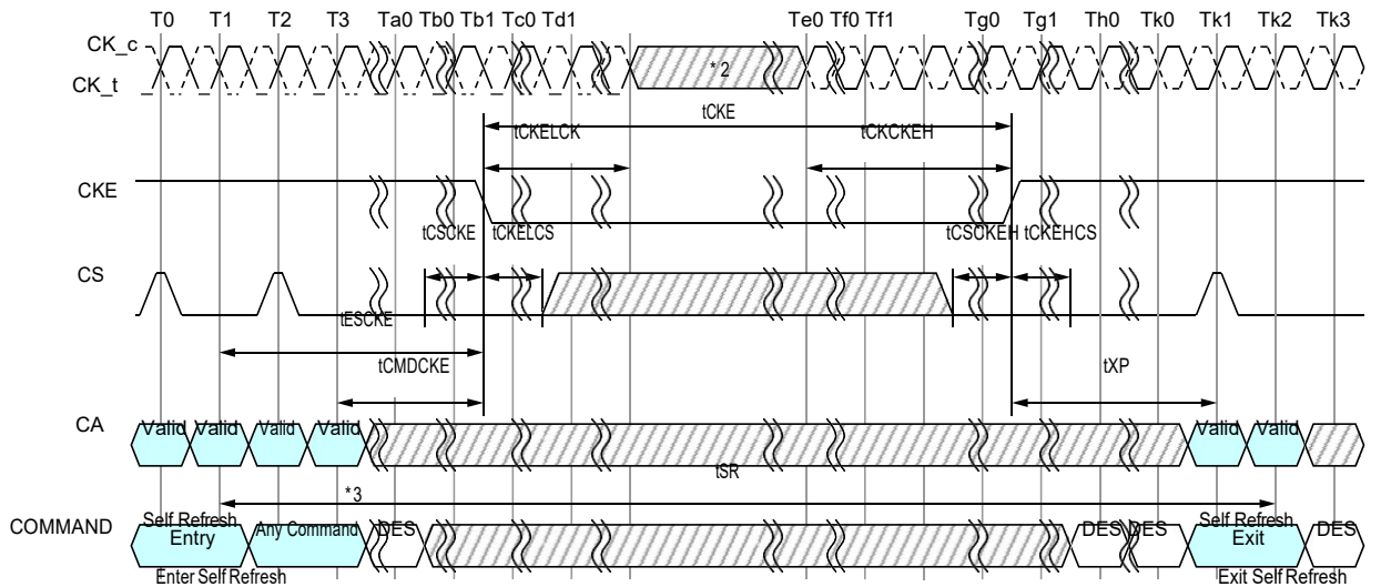
Figure - Self Refresh Entry/Exit Timing with Power Down Entry/Exit
