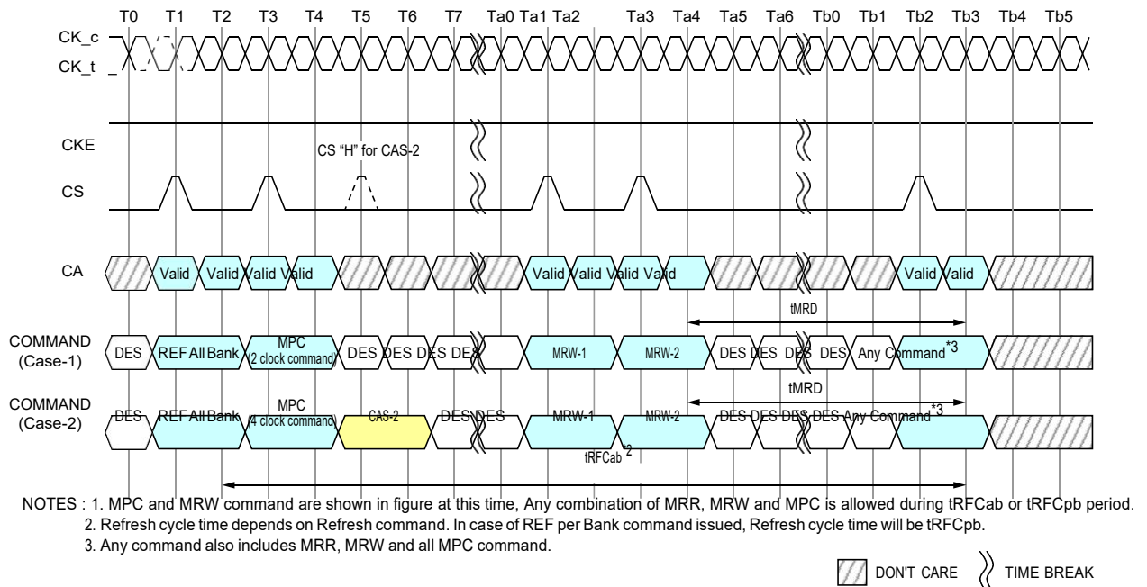
Figure - MRR, MRW and MPC Commands Issuing Timing during tRFC
