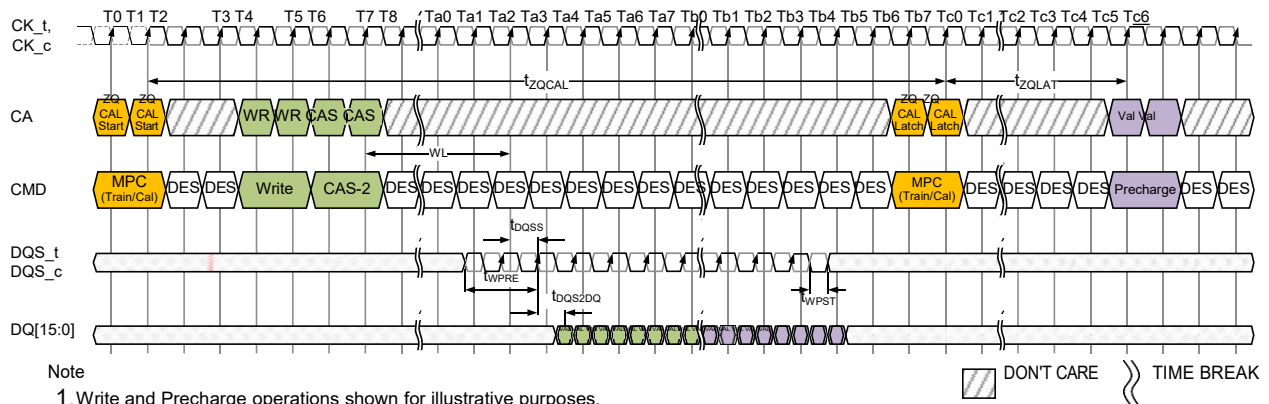
Figure - ZQCal Timing
