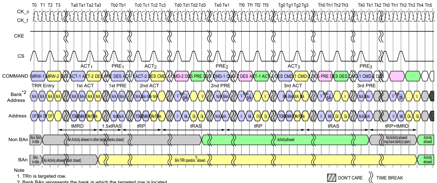
Figure - TRR Mode Timing Example
