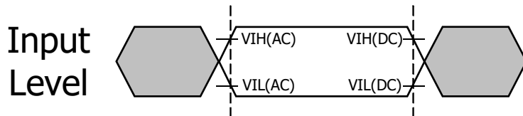
Figure - Input AC timing definition for CKE
