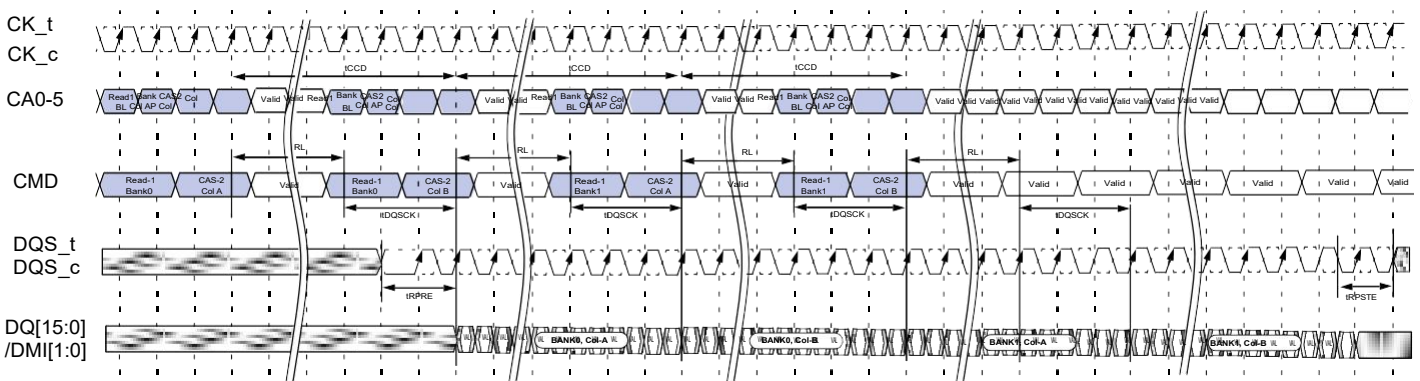
Figure - Seamless Burst Read. BL=16, Toggling tRPRE, Extended tRPST
