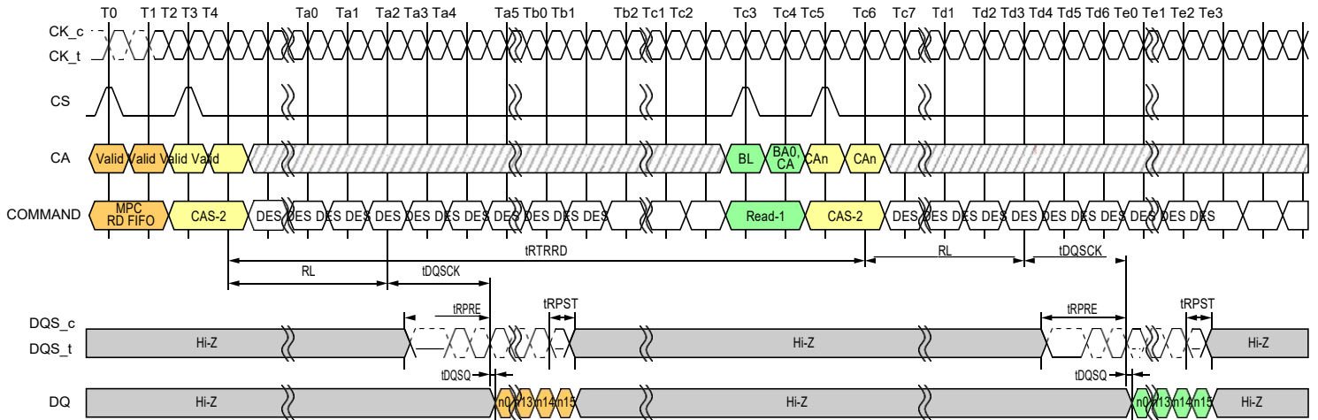
Figure - MPC [Read FIFO] to Read Timing
