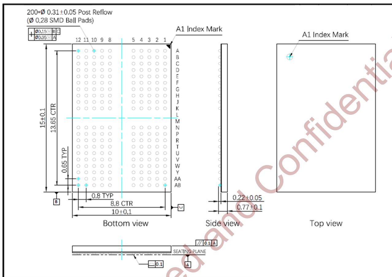
Figure 2-1 200-Ball x32 Discrete FBGA Package Dimension
