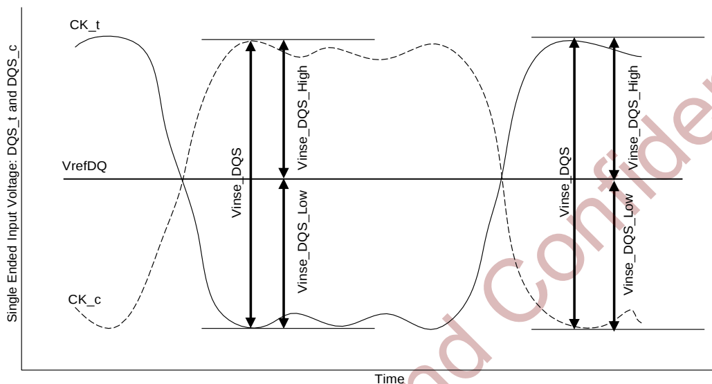
Figure 5-13 DQS Single-Ended Input Voltage
