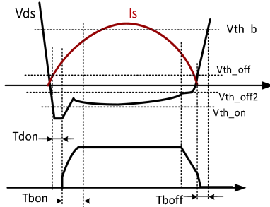
Figure 1 ON/OFF control logic
