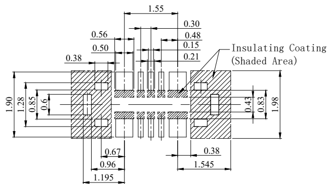
RECOMMENDED PCB LAYOUT DIMENSIONAL TOLERANCE: \pm 0.02
