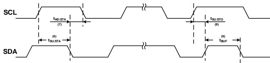
Figure 3 The timing relationship between START and STOP state
