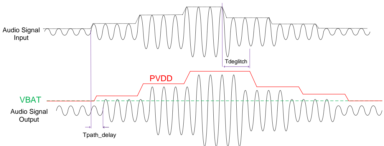
Figure 3 Boost Circuit Behavior in Smart Boost Mode
