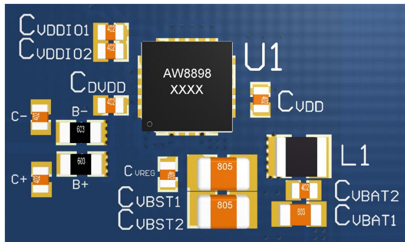
Figure 10 AW8898QNR External Components Placement
