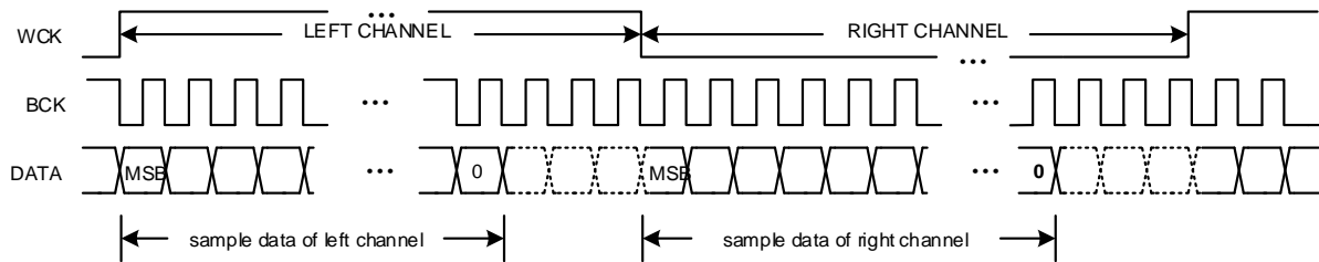
Figure 8 I 2 S Timing for Left-Justified Mode
