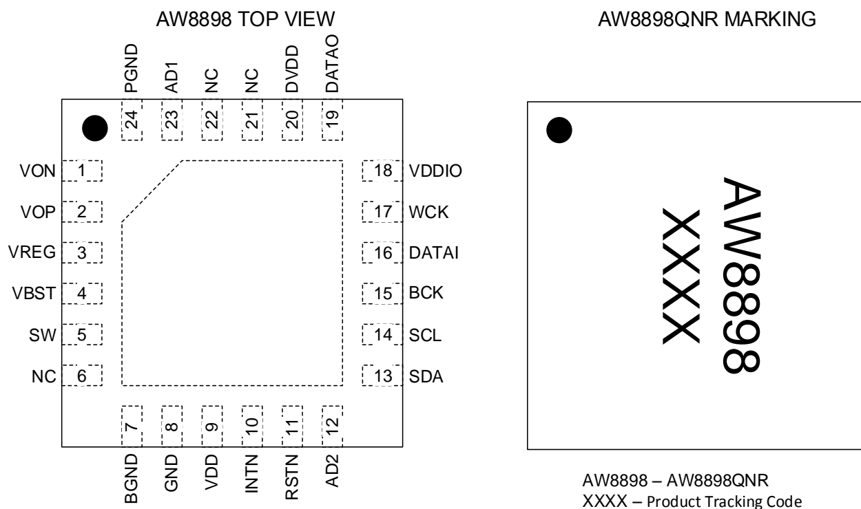
Figure 1 AW8898QNR pin diagram top view and device marking
