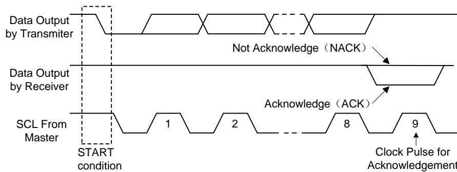
Figure 6 I²C ACK Timing
