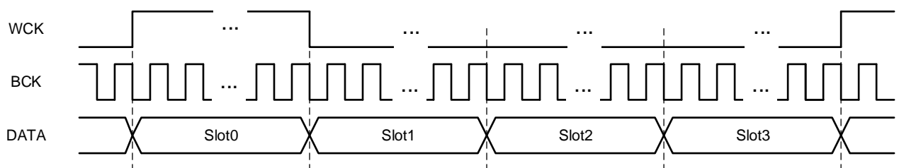
Figure 1 TDM Timing
