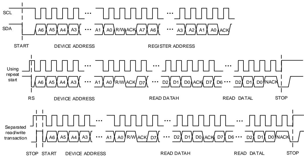
Figure 8 I 2 C Read Byte Cycle
