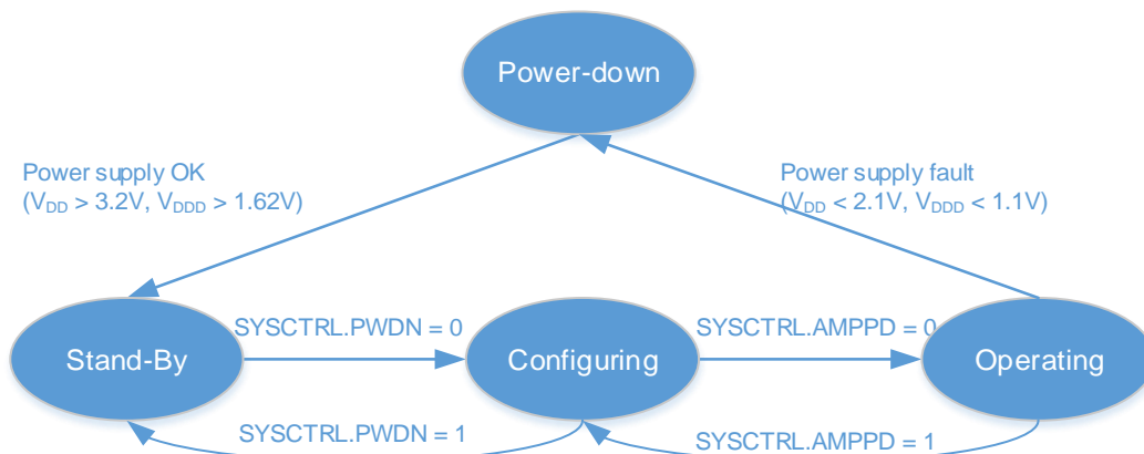
Figure 5 Device operating modes transition
