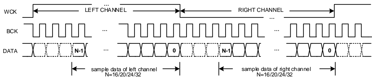
Figure 9 I 2 S Timing for Right-Justified Mode
