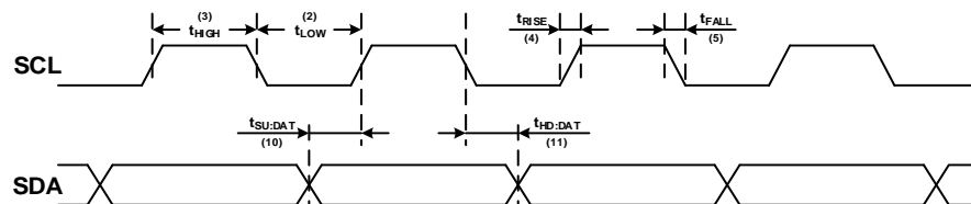
Figure 2 SCL and SDA timing relationships in the data transmission process
