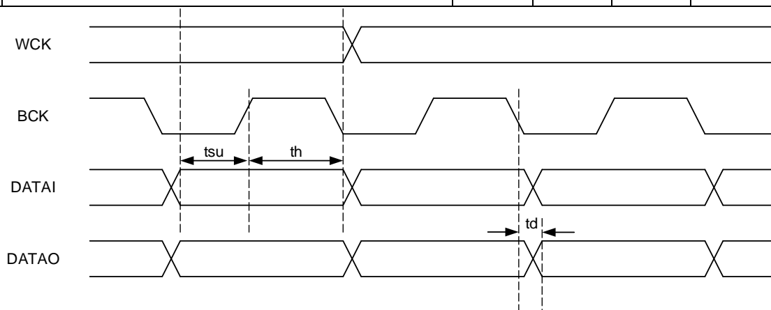
Figure 4 Digital Audio Interface Timing
