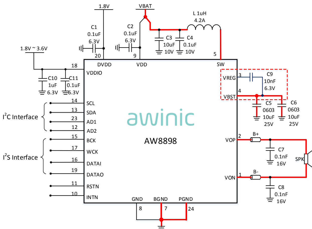
Figure 1 AW8898 Application Circuit
