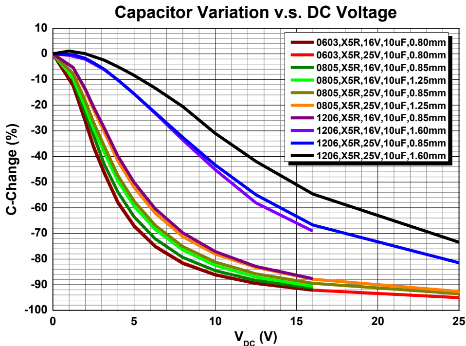
Figure 9 Different types of capacitive voltage stability
