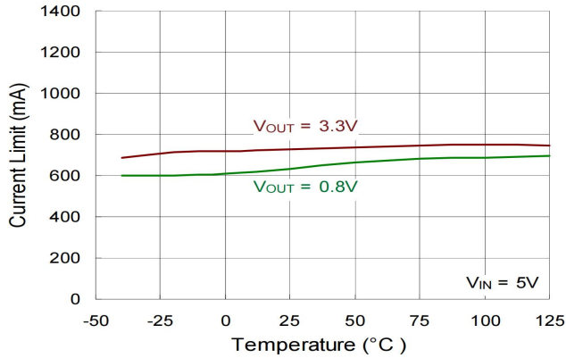
Fold-Back Current Limit vs. Temperature
