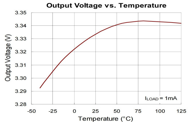
Figure 4. Temperature Coefficient of Adjustable Output Voltage
