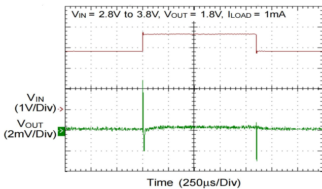
Line Transient
