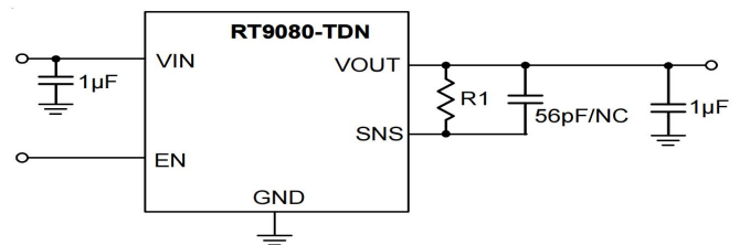
Figure 5. Fine Adjustable Output Voltage Application Circuit
