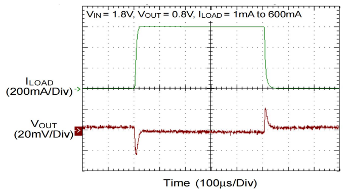
Load Transient
