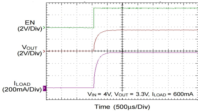
Power On from EN
