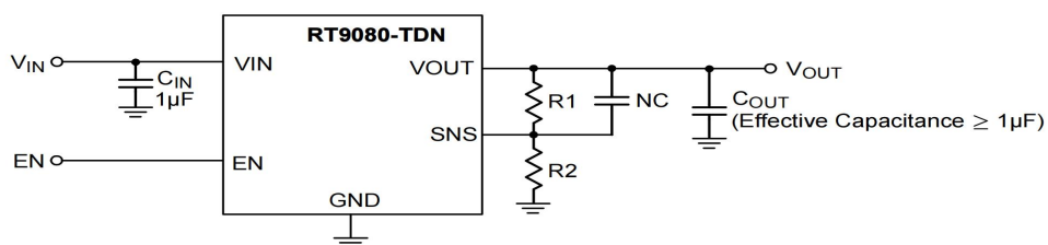
Figure 3. Adjustable Output Voltage Application Circuit
