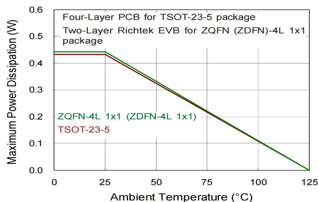
Figure 6. Derating Curve of Maximum Power Dissipation
