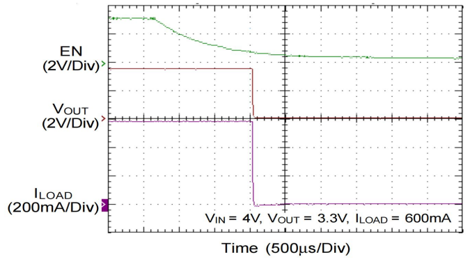
Power Off from EN
