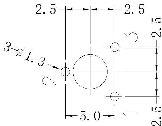
PC板固定孔圖 P.C.B. MOUNTING HOLE DETAIL
