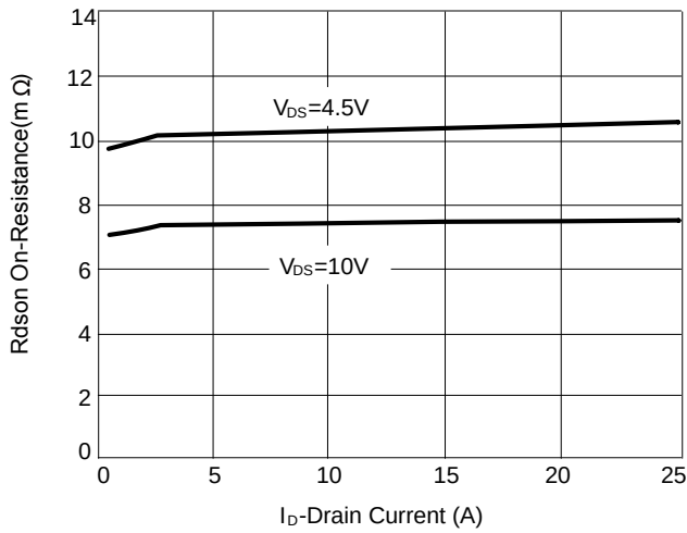
Figure 3: Rdson-Drain Current
