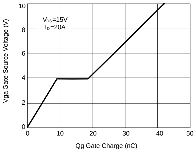
Figure 6: Gate Charge
