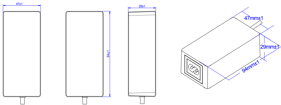
8字尾 IEC320-C8
