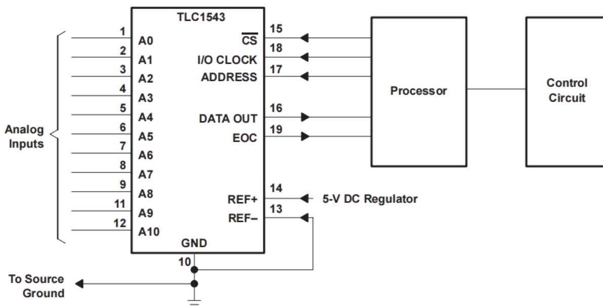
Figure 16. Serial Interface
