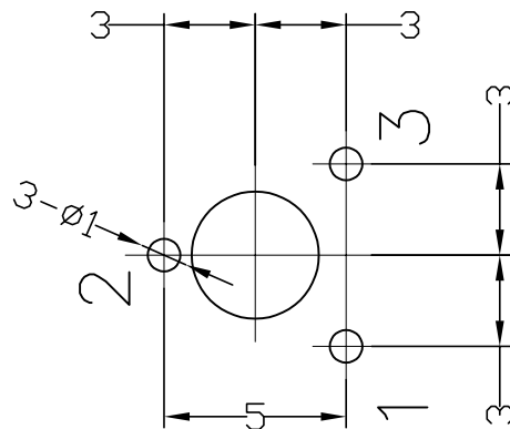
PC板固定孔圖 P.C.B. MOUNTING HOLE DETAIL
