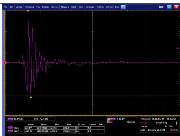
IEC6100-4-2 -8kV IO-GND
