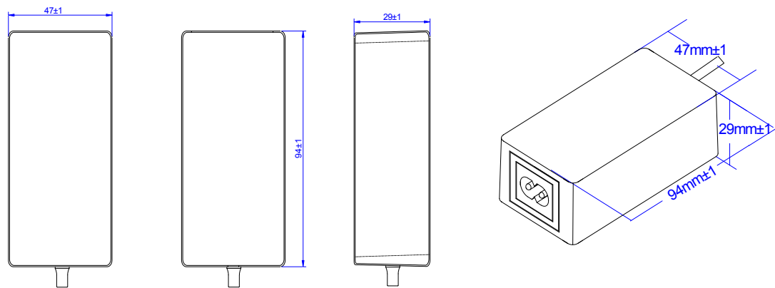
8字尾 IEC320-C8
