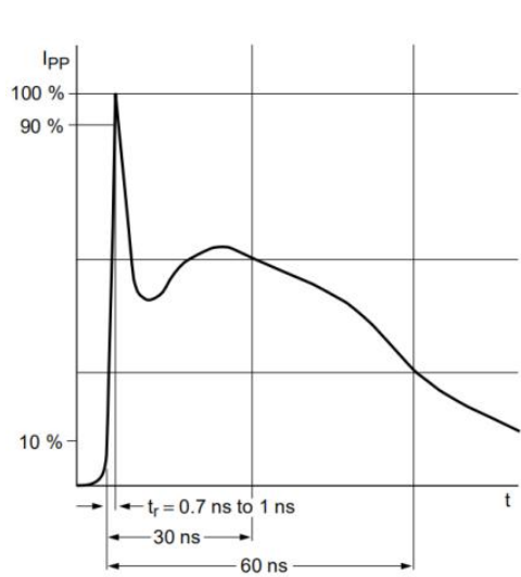
IEC61000-4-2 Waveform
