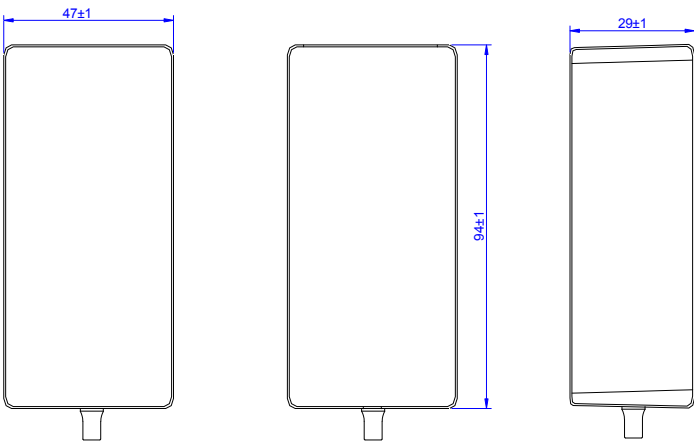
8字尾 IEC320-C8
